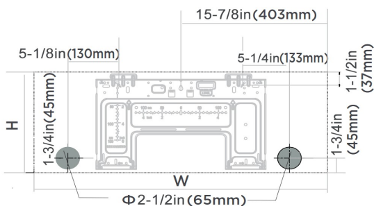
Indoor unit dimensions(WxH): 31-3/4in(806mm)x11-5/8in(296mm)
