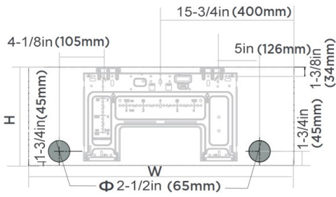
Indoor unit dimensions(WxH): 28-3/4in(729mm)x11-1/2in(293mm)
