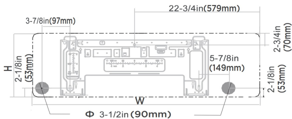
Indoor unit dimensions(WxH): 42-5/8in(1082mm)x13-1/2in(338mm)
