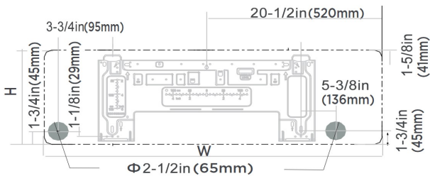
Indoor unit dimensions(WxH): 38-1/4in(971mm)x12-5/8in(321mm)
